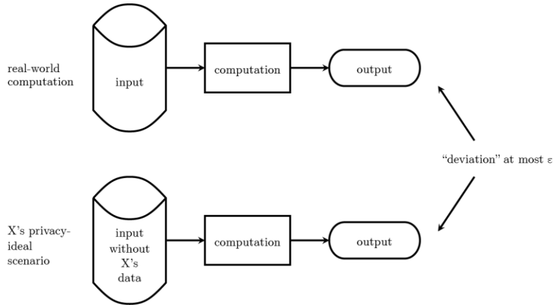
Figure 4: Differential privacy.
