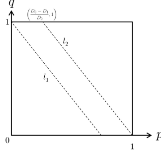
Figure 2: The strategy space for agent B and the corresponding best response of A . When B plays a (p, q) -point above line \ell_1 , then A sets x = 1 ; When B plays a (p, q) -point above line \ell_2 , then A sets y = 1 .
