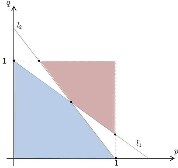
Figure 3: The 4 regions created by the lines l_1 and l_2 , and the 5 intersection points of the two lines and the borders of the squares.
